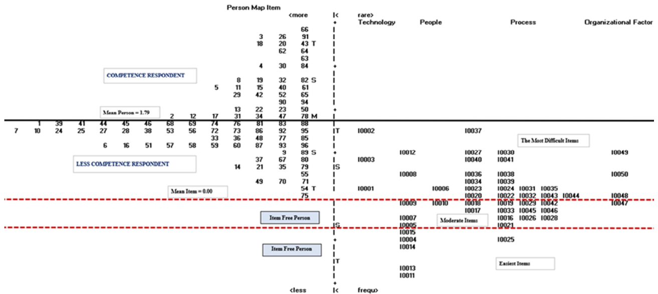
Fig. 6 Person Item Distribution Map
