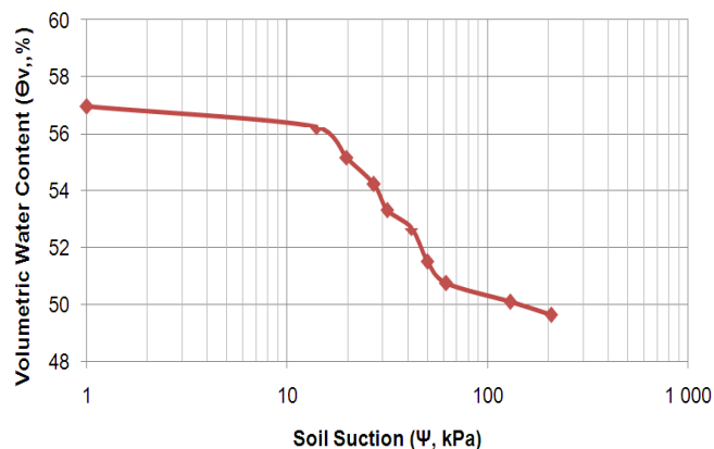
Fig. 12 Graph volumetric of water content versus clay soil suction from sample c1
