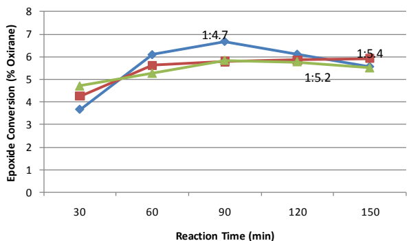
Fig. 5. Epoxidation with peracetic acid at 60°C. The concentration was a ratio of acetic acid to H 2 O 2 .
