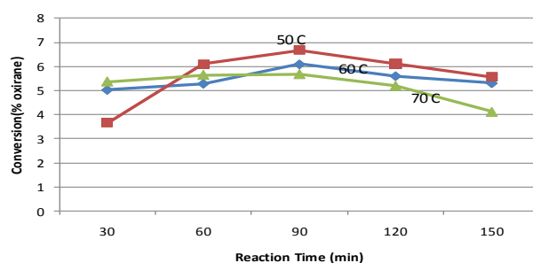
Fig 3. Epoxidation with peracetic acid with temperature reaction 50, 60, and 70°C
