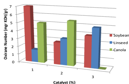
Fig. 1. Catalyst for epoxidation at 60°C
