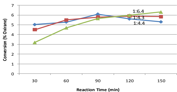
Fig. 4 Epoxidation with peracetic acid at 50°C. The concentration was a ratio of acetic acid to H 2 O 2 .
